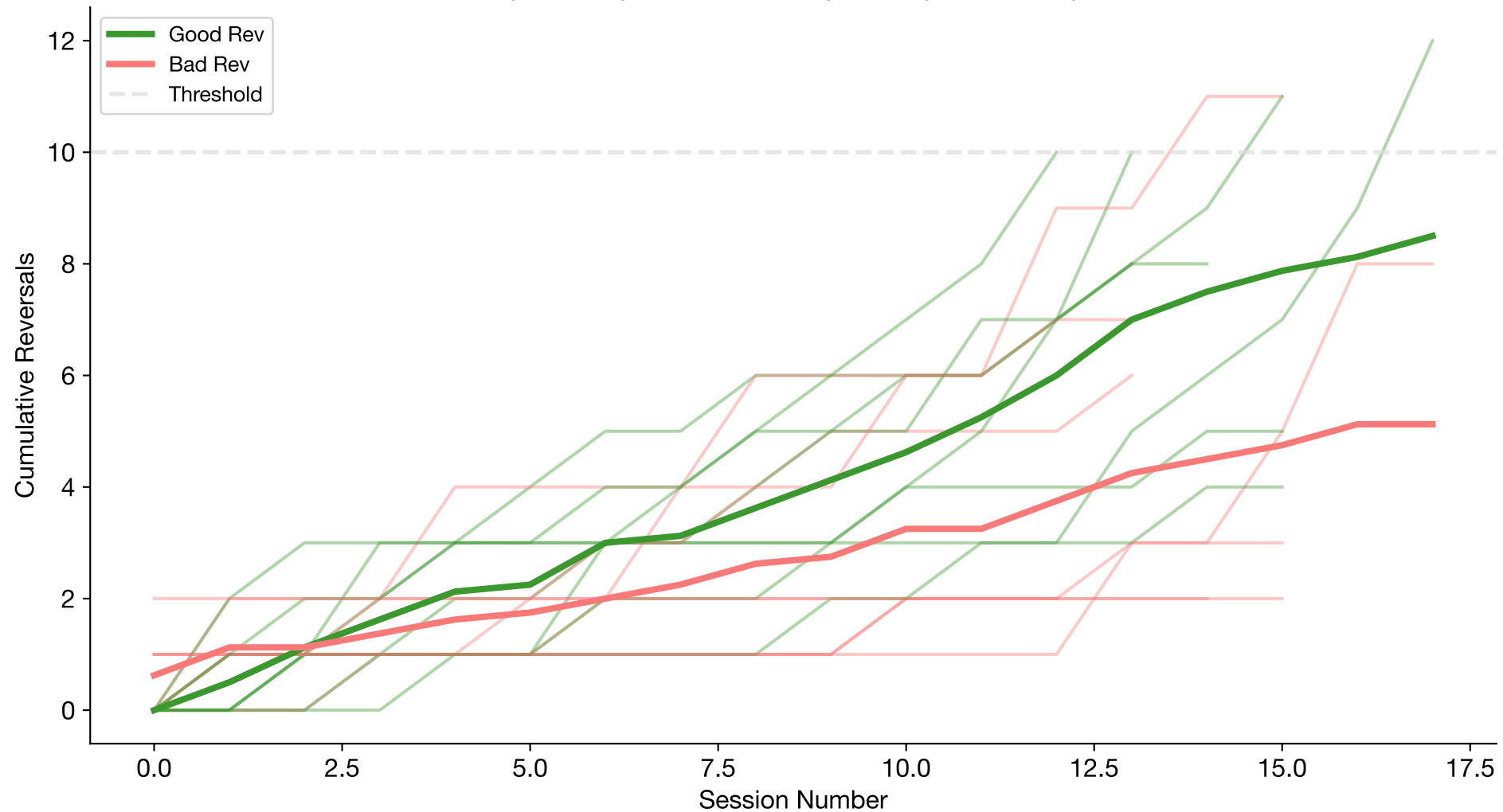
Cumulative Good and Bad Reversals Over Time (n=8 subjects; sessions per subject=13–18)
